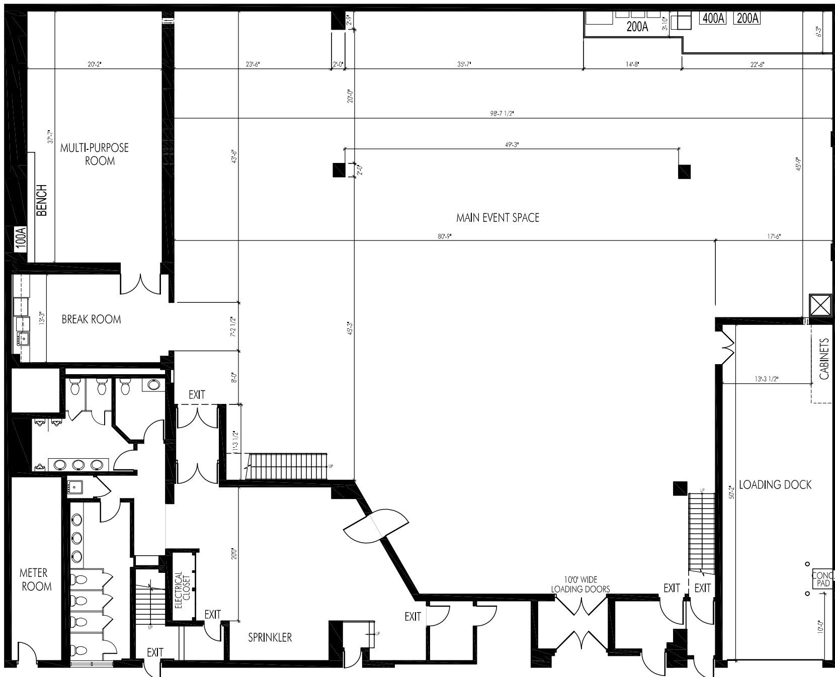
1 GROUND FLOOR PLAN NOT TO SCALE
